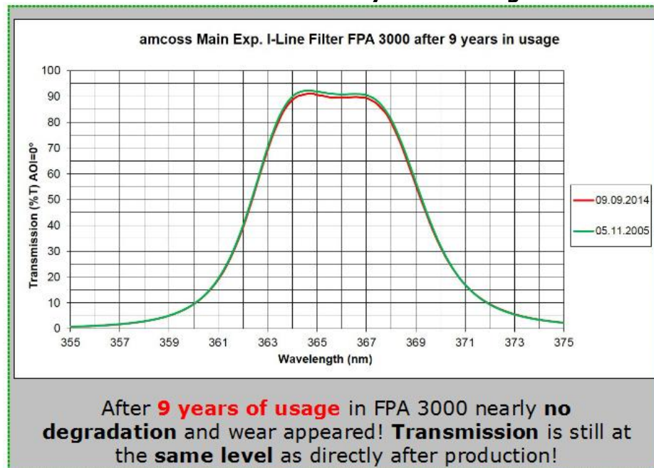
amcos filter after 9 years of usage
